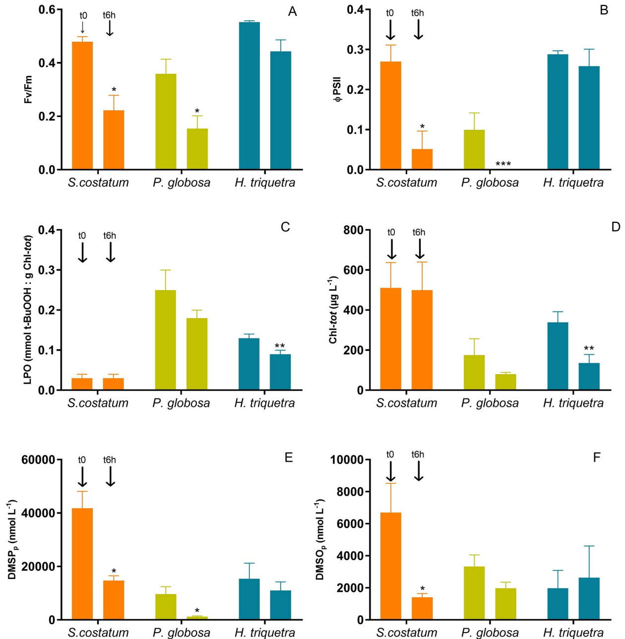
Fig. 5. Evolution of (A) Maximum quantum yield of PSII (Fv/Fm), (B) Effective photochemical quantum yield of PSII (ΦPSII), (C) Lipid Peroxidation (LPO) (mmol t-BuOOH:g Chl-tot), (D) Chlorophyll-tot (Chl-tot) concentration (μg L -1 ), (E) the DMSP p concentration (nmol L -1 ), and (F) the DMSO p concentration (nmol L -1 ) with 25 μmol L -1 MSB during 6 h for the three species S. costatum , P. globosa and H. triquetra . Error bars represent SD calculated from triplicates biological samples. Asterisks denote significant differences between the two time-point (* P < 0.05; ** P < 0.01; *** P < 0.001).
