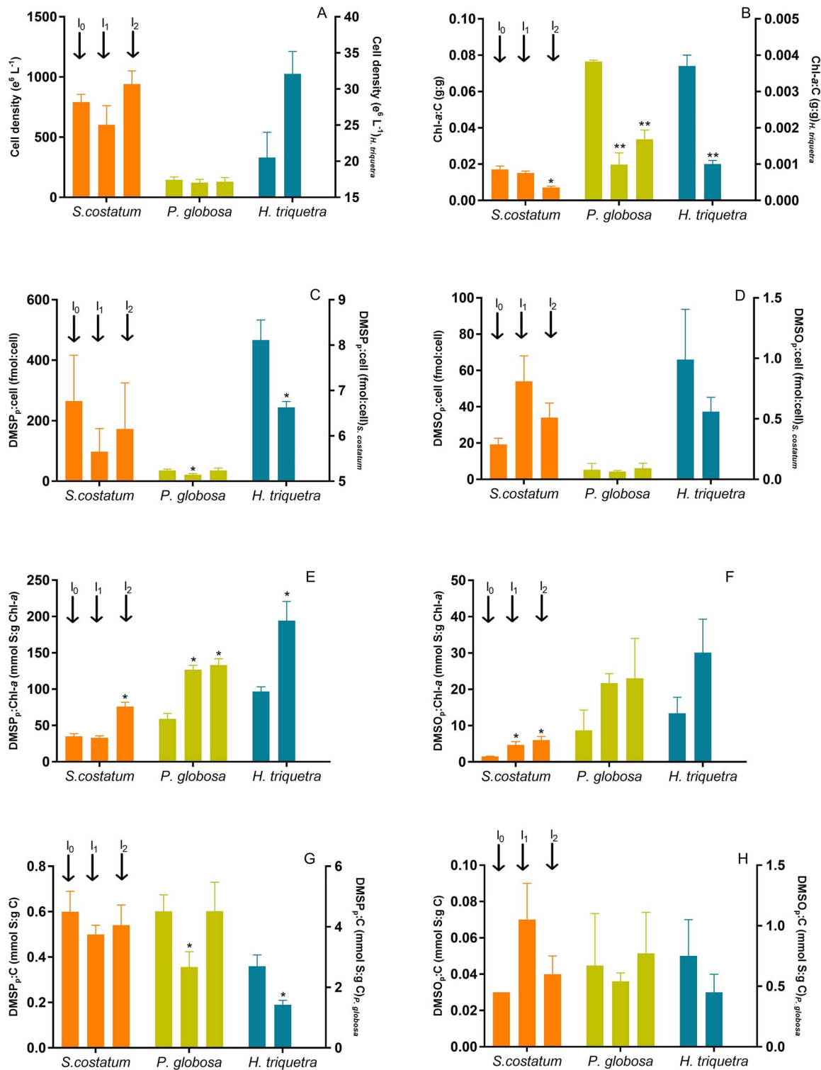
Fig. 2. Evolution of (A) Cellular density ( \times 10^6 \text{ cells L}^{-1} ); (B) Cellular Chlorophyll- a content (Chl- a :C) (g:g), (C) the DMSP p :Cell ratio (fmolS:cell); (D) the DMSO p :Cell ratio (fmolS:cell); (E) the DMSP p :Chl- a ratio (mmol S:g Chl- a ), (F) the DMSO p :Chl a ratio (mmol S:g Chl- a ); (G) the DMSP p :C ratio (mmol S:g C), (H) the DMSO p :C ratio (mmol S:g C) at three light intensities of 100 (left bar), 600 (central bar) and 1200 (right bar) \mu\text{mol photon m}^{-2} \text{s}^{-1} during the long-term HL treatment for the three species S. costatum , P. globosa and H. triquetra . Error bars represent SD calculated from triplicates biological samples. Asterisks denote significant differences between the control and the light intensity considered (* P < 0.05 ; ** P < 0.01 ; *** P < 0.001 ).
