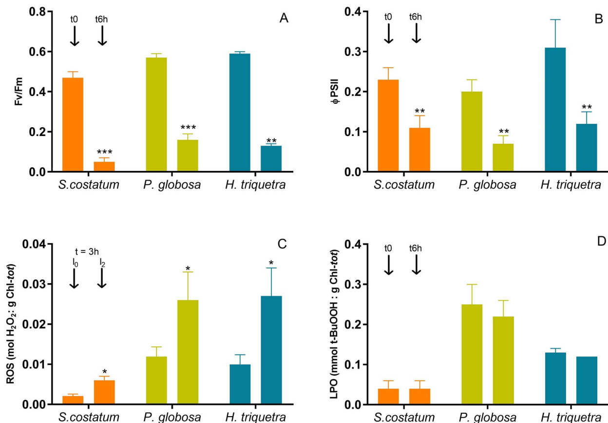
Fig. 1. Evolution of (A) Maximum quantum yield of PSII ( F_v/F_m ), (B) Effective photochemical quantum yield of PSII ( \Phi_{PSII} ), (C) Reactive oxygen species (ROS) ( \text{mol H}_2\text{O}_2 \cdot \text{g Chl-tot}^{-1} ) at the beginning and after 3 h, (D) Lipid peroxidation (LPO) ( \text{mmol t-BuOOH} \cdot \text{g Chl-tot}^{-1} ) with increasing light intensity from 100 to 1200 \mu\text{mol photon m}^{-2} \text{s}^{-1} during 6 h for the three species S. costatum , P. globosa and H. triquetra . ROS analysis was performed after 3 h. Error bars represent SD calculated from triplicates biological samples. Asterisks denote significant differences between the time point 0 and 6 h, or after 3 h between the control conditions at 100 and 1200 \mu\text{mol photon m}^{-2} \text{s}^{-1} (* P < 0.05 ; ** P < 0.01 ; *** P < 0.001 ).
