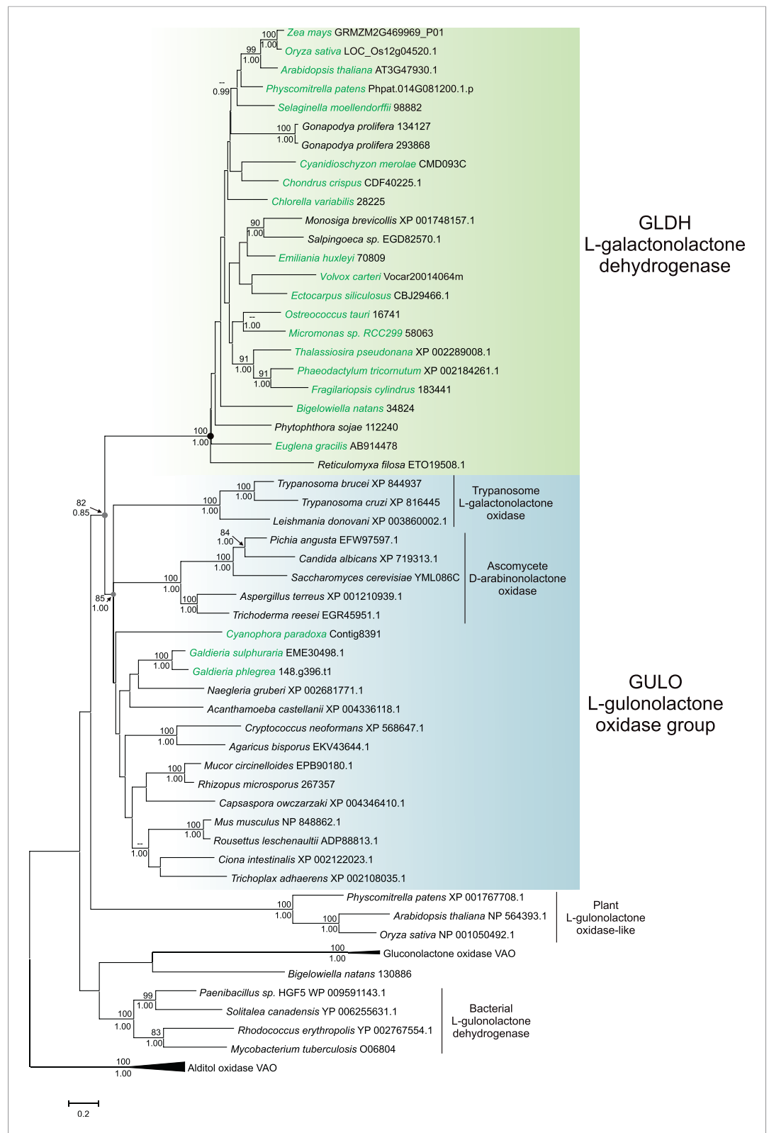
Figure 3. Phylogenetic analysis of L-gulonolactone oxidase and L-galactonolactone dehydrogenase. A maximum likelihood phylogenetic tree demonstrating the relationships between aldolactone oxidoreductases involved in ascorbate biosynthesis. A multiple sequence alignment of 263 amino acid residues was used with alditol oxidases from the vanillyl alcohol oxidase (VAO) family acting as the outgroup. Photosynthetic organisms are shown in green. Figure 3. continued on next page
