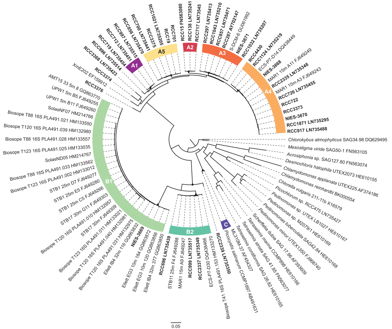
Figure 2 ML tree inferred from nuclear 16S rRNA sequences belonging to prasinophytes clade VII. Nodes supported by NJ, ML and Bayesian methods are shown by a solid dot (●).
