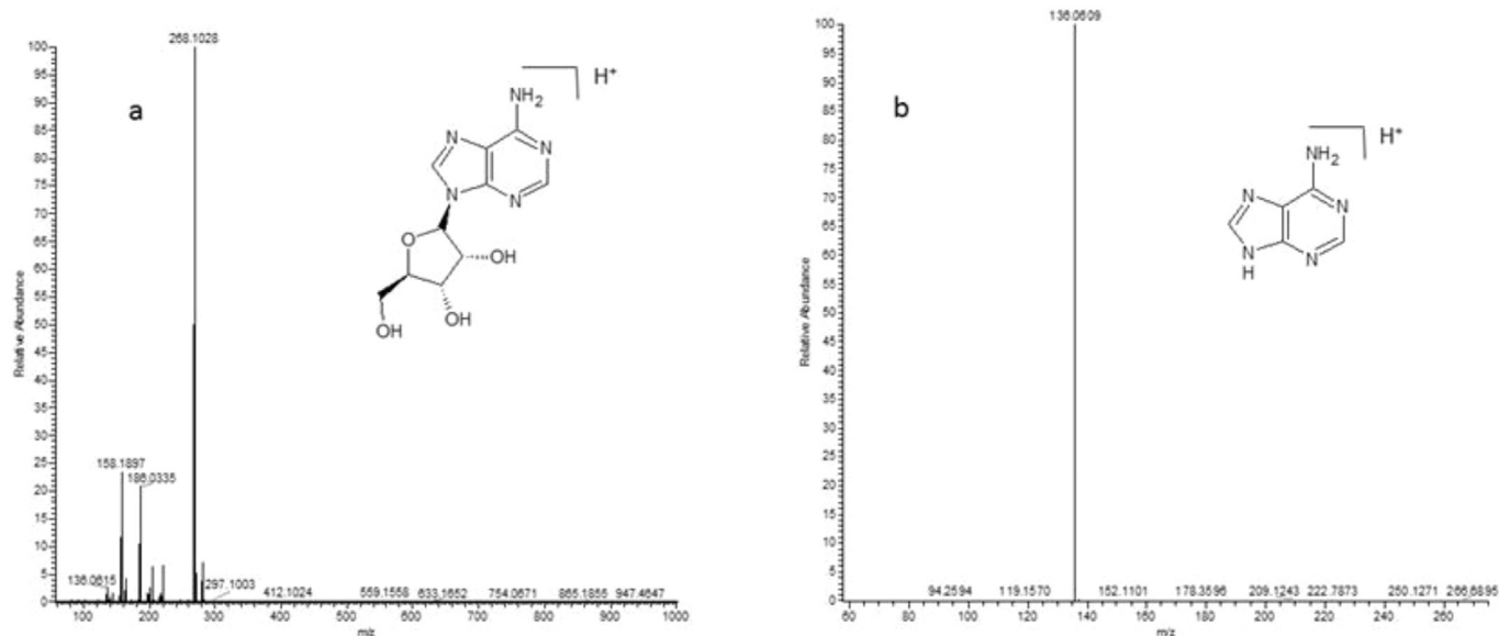
Fig. 4. Mass spectra for a) adenosine and b) 1H-Imidazo[4,5-d]pyridazin-4-amine detected in cultures of Emiliana huxleyi at the time of harvesting.
