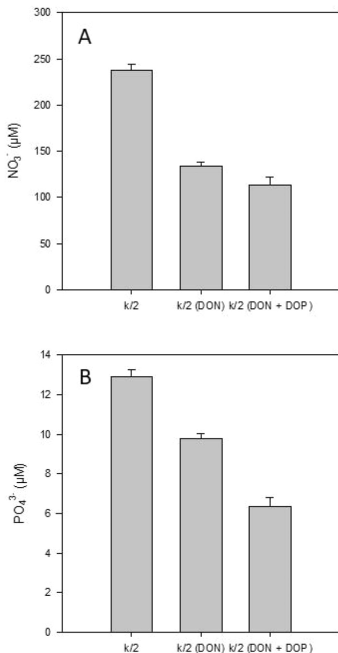
Fig. 1. Concentrations of A, dissolved nitrate; B, dissolved phosphate in 6 L cultures of Emiliana huxleyi at the time of harvesting.
