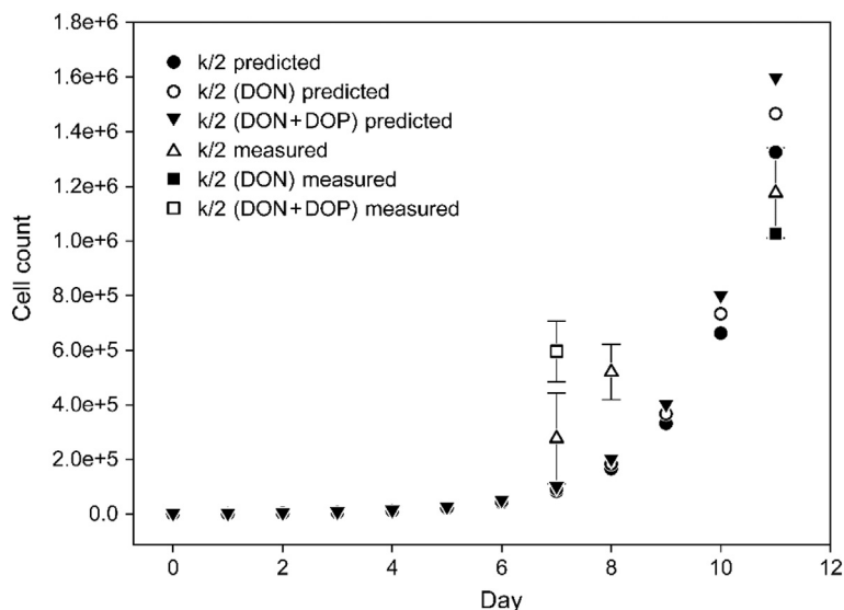
Fig. 3. Measured cell counts for Emiliana huxleyi cultured in 6 L volumes without replenishment in: k/2 culture medium ( \Delta ), k/2 medium containing DON ( \blacksquare ) and k/2 medium containing DON + DOP ( \square ). Predicted growth rates for cultures were based on cell counts at the time of sub-culturing to 6 L and assumed one cell division per day ( \bullet = k/2_{\text{predicted}} , \circ = k/2 \text{ DON}_{\text{predicted}} , \blacktriangledown = k/2 \text{ DON + DOP}_{\text{predicted}} ).
