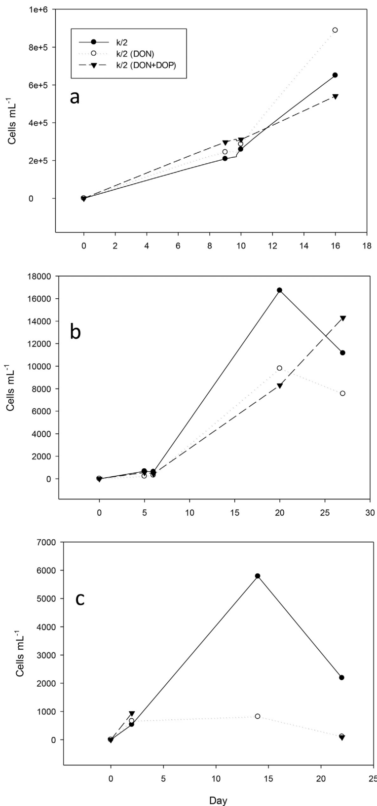
Fig. 2. Measured cell counts for Emiliana huxleyi (a); Prorocentrum minimum (b); Chaetoceros sp. (c). The culture volume was 2 L and the culture vessels amended with fresh medium (0.5 L) at intervals during the culturing period.
